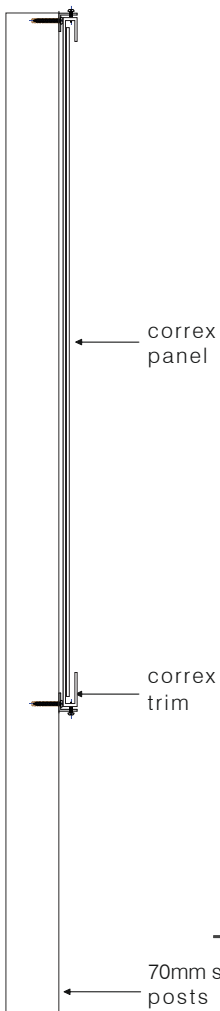
Sign B One aluminium wall mounted A0 correx sign, Non illuminated. Sizes 1260 x 910mm, G/Cl - 300mm, D - 25mm.
