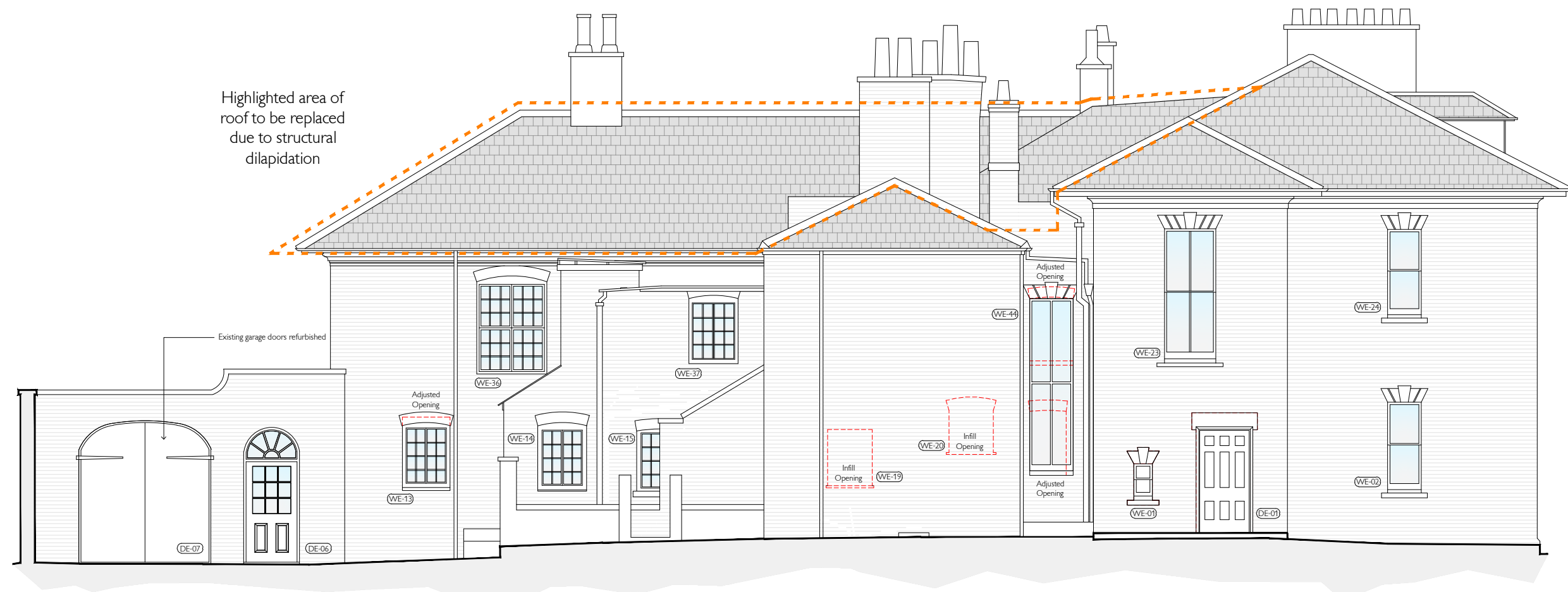
Front Elevation (Facing North)
