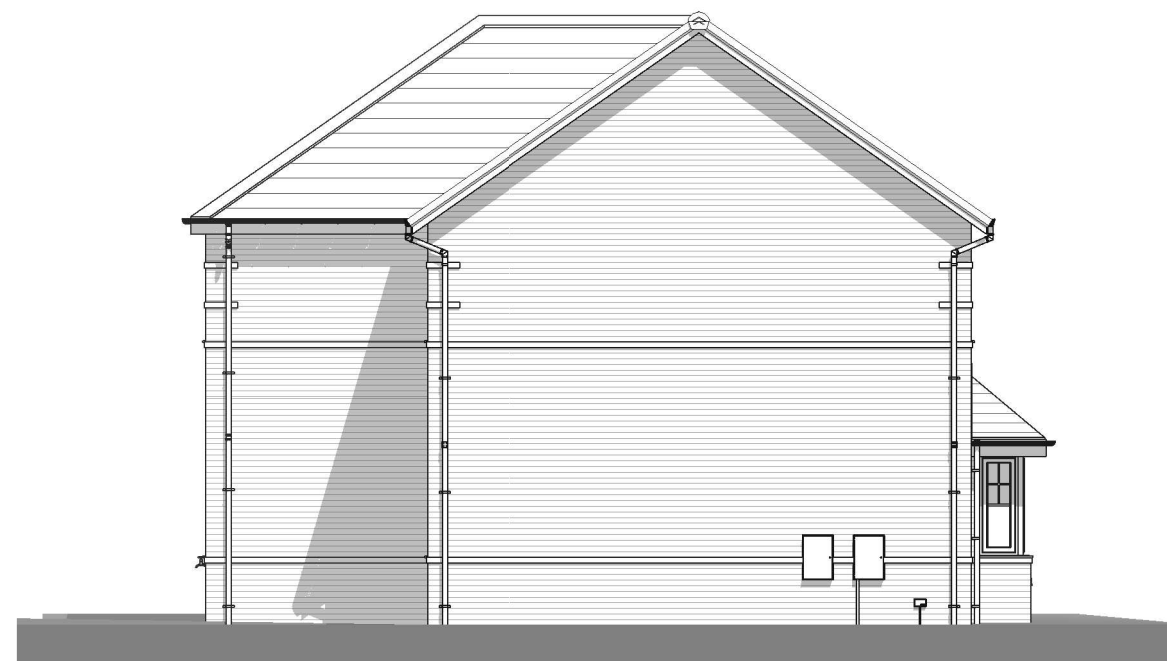
Left Elevation. 1 : 100
