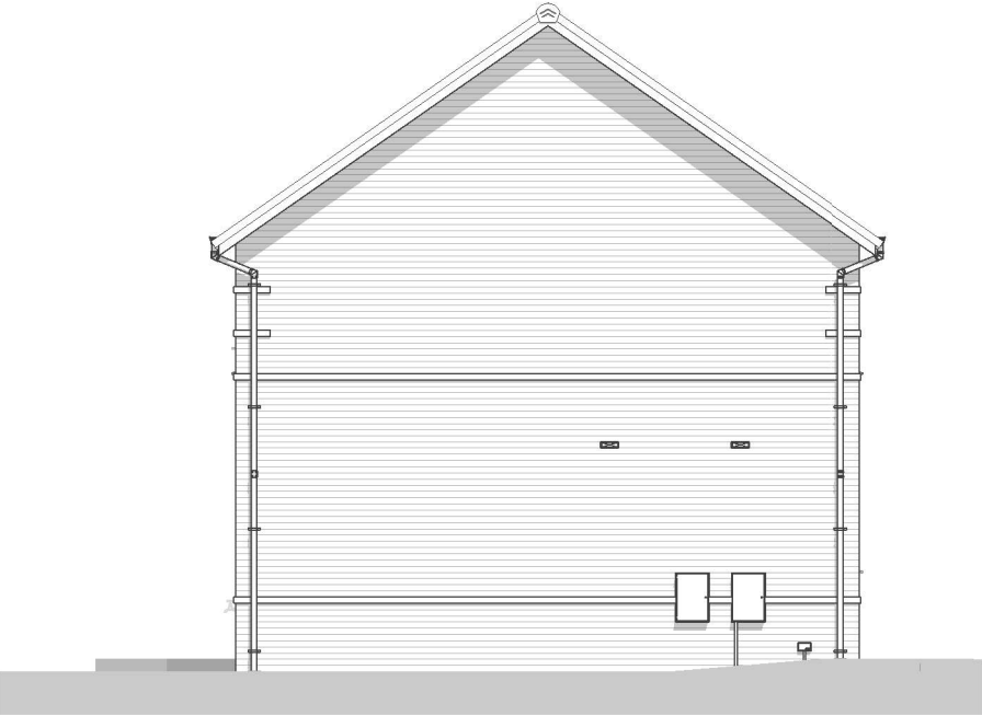
Left Elevation. 1 : 100
