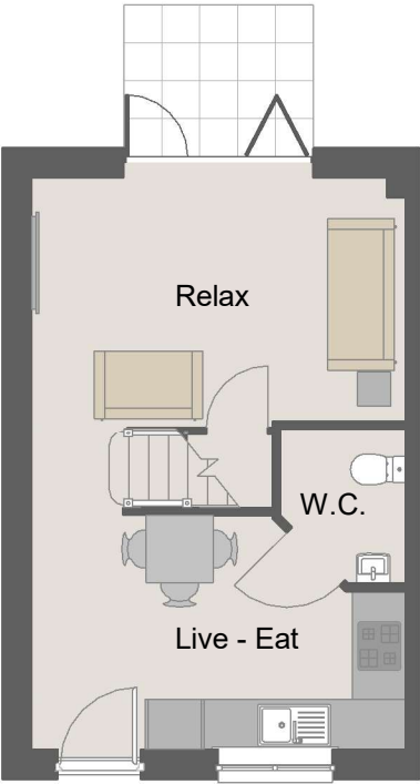
Ground Floor. 1 : 100
