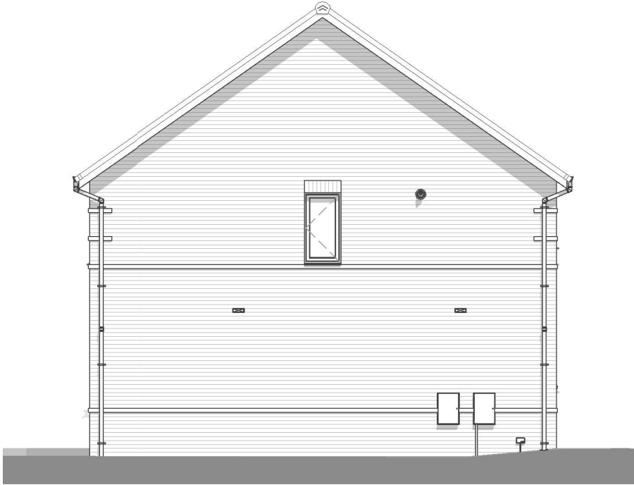
Left Elevation. 1 : 100
