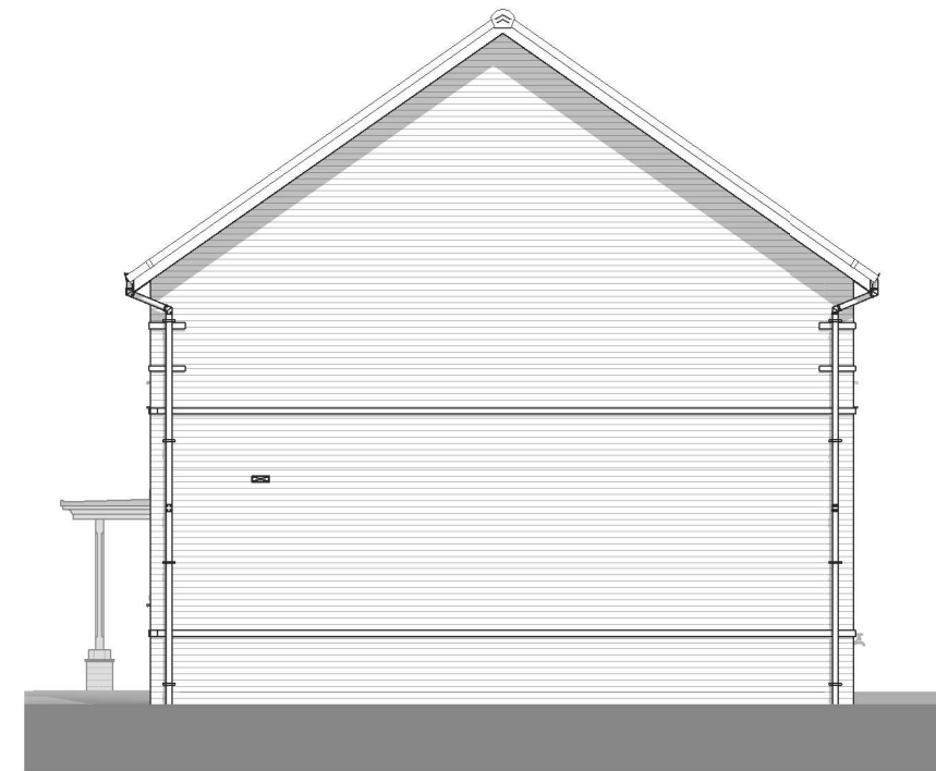
Right Elevation. 1 : 100
