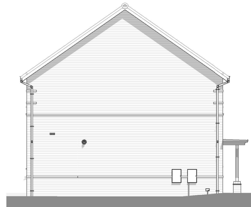
Left Elevation. 1 : 100
