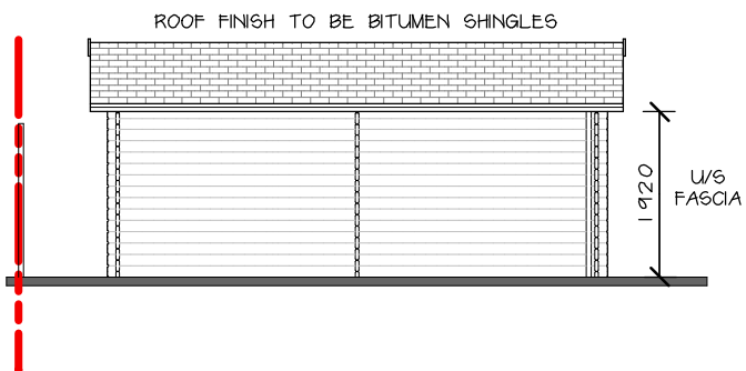
WORKSHOP SIDE ELEVATION 1:100
