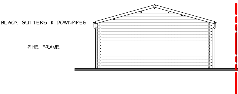
WORKSHOP REAR ELEVATION 1:100
