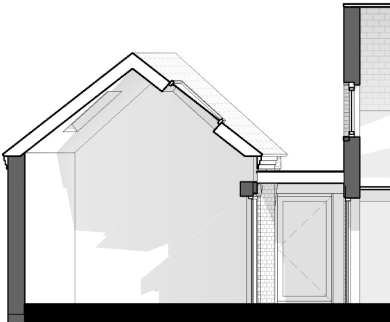
Proposed Section A - A Scale 1 : 100
