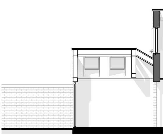
Proposed Section B - B Scale 1 : 100
