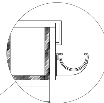
BUILDING 2 - EAVES DETAIL
