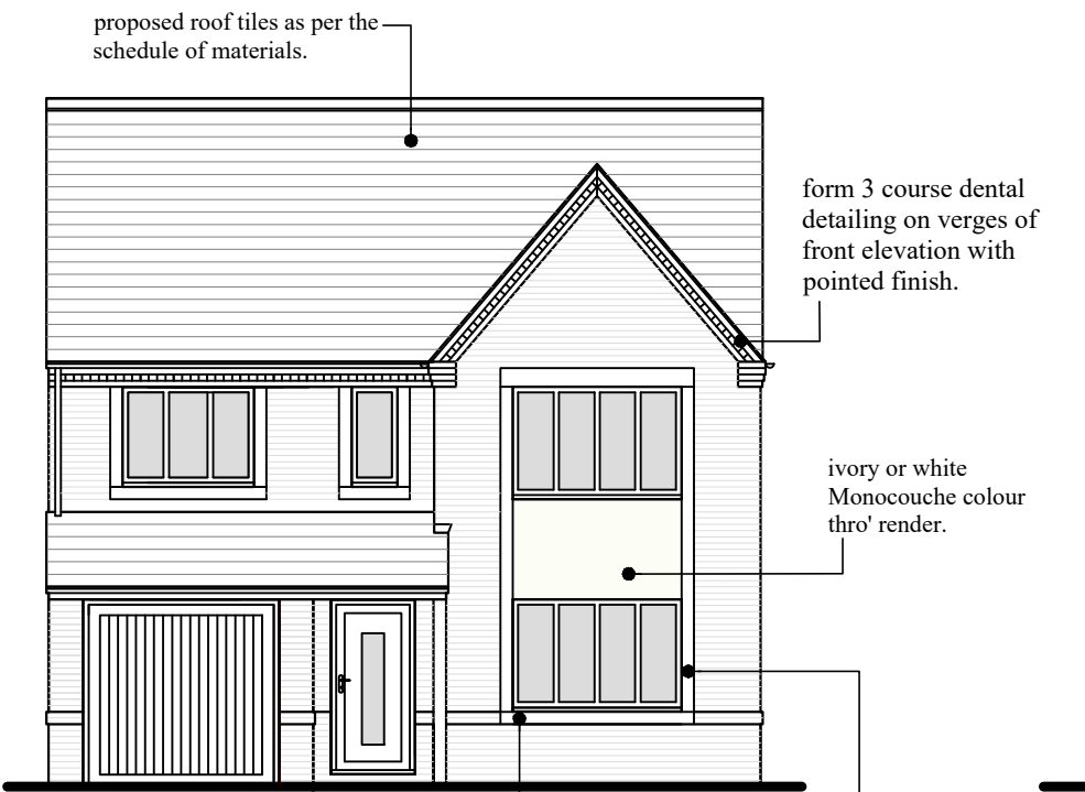
FRONT ELEVATION
