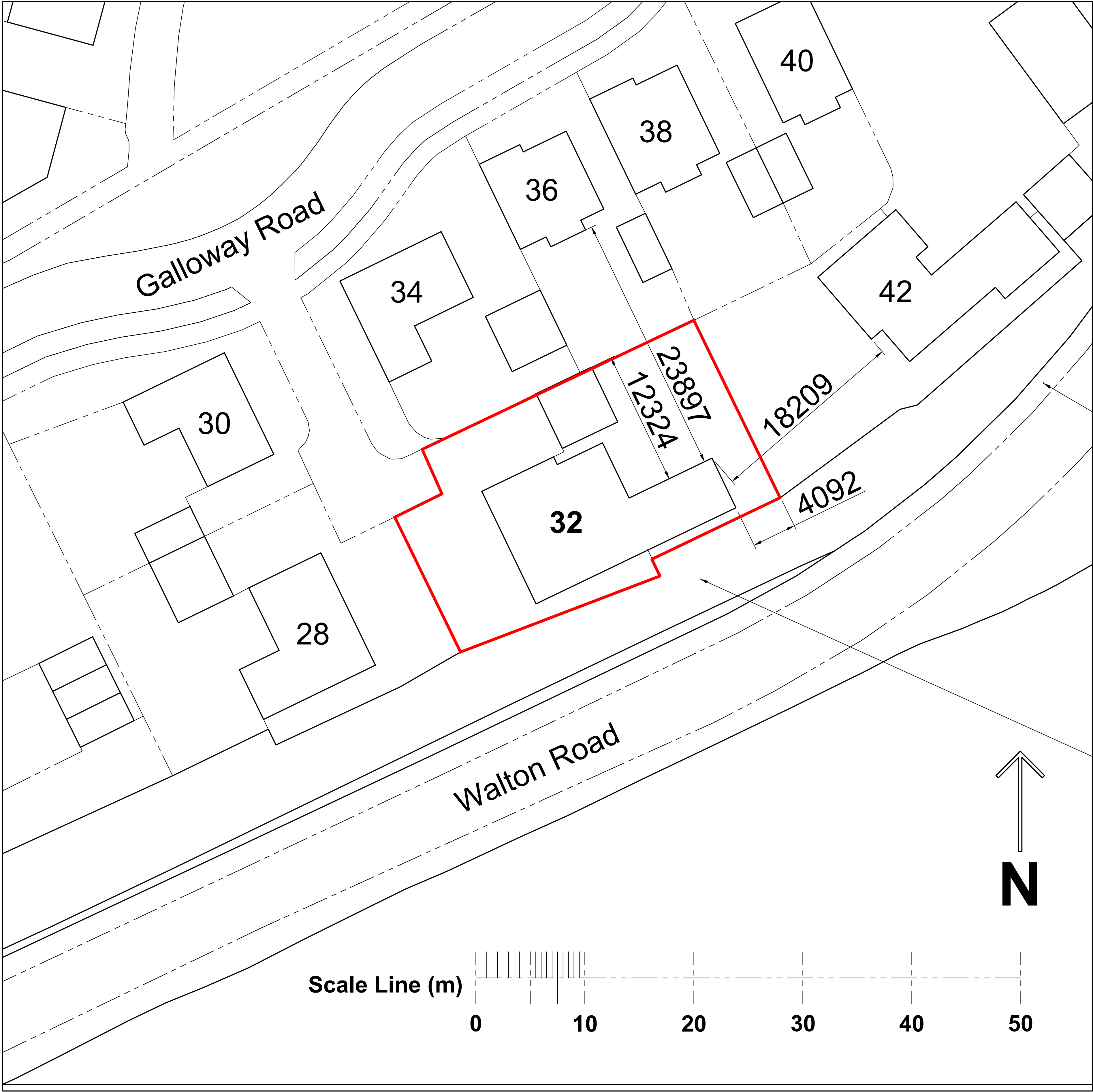
Site / Block Plan (Scale 1:200)
