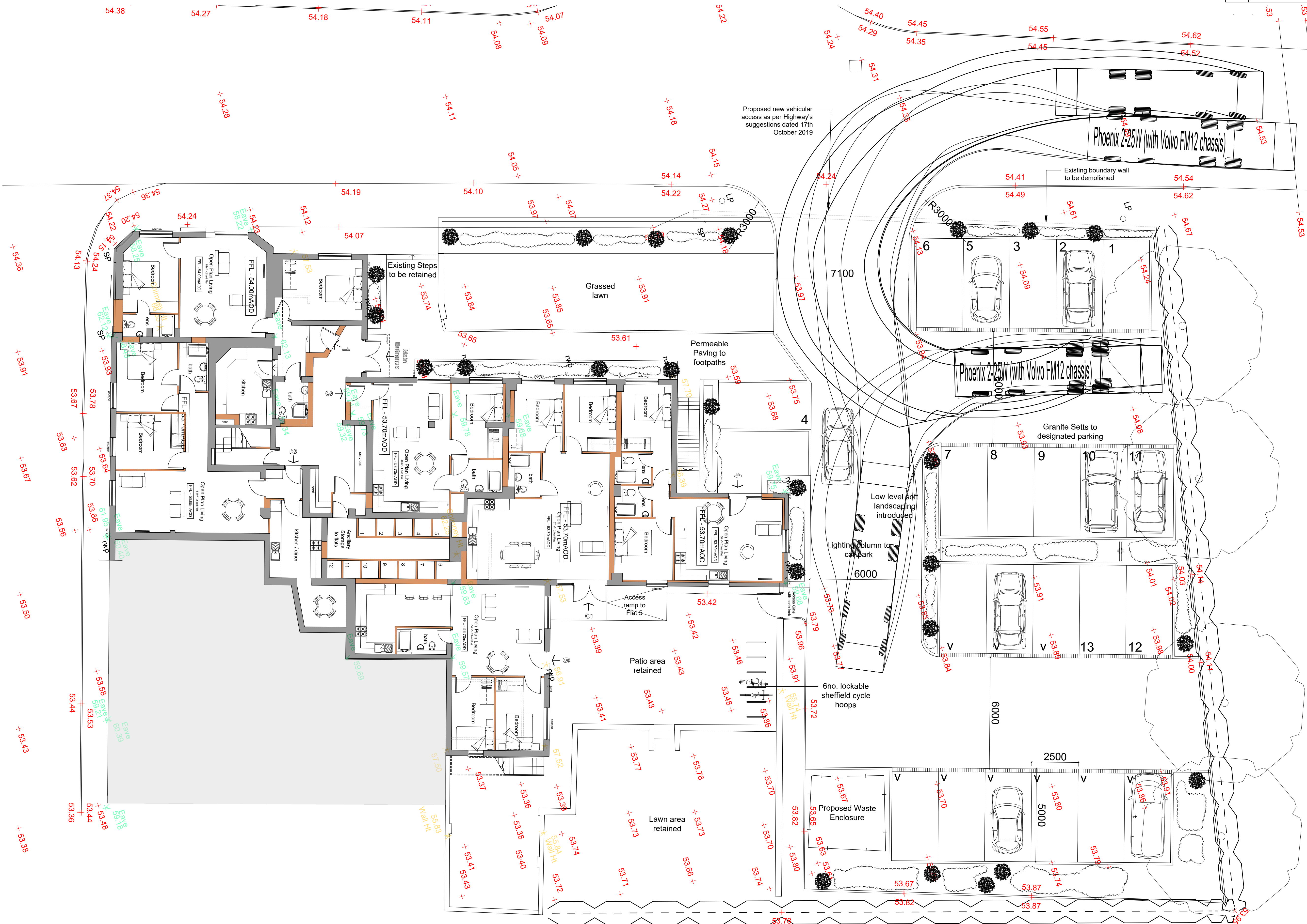
Proposed Site Layout Scale 1:100
