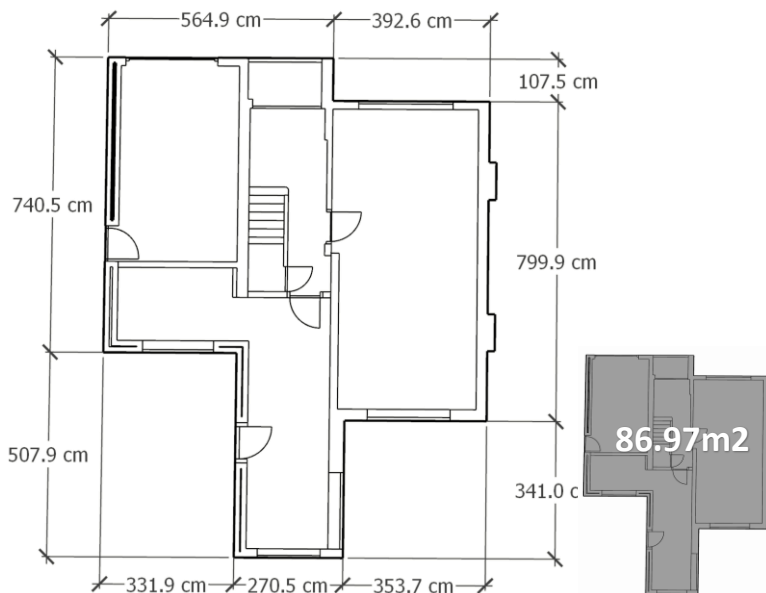
Existing Floor Plans
