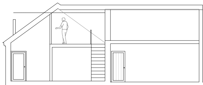
SECTION A - A @1:50
