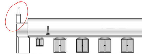
WEST ELEVATION @1:100
