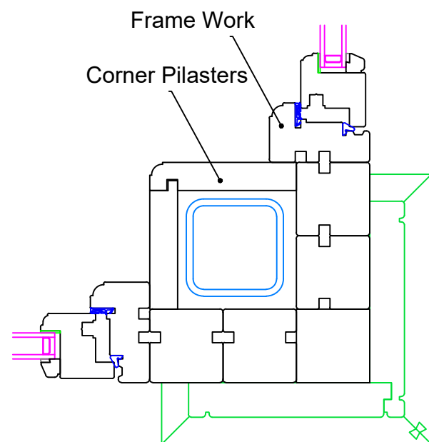
PLAN VIEW OF CORNER PILASTERS Scale 1:5
