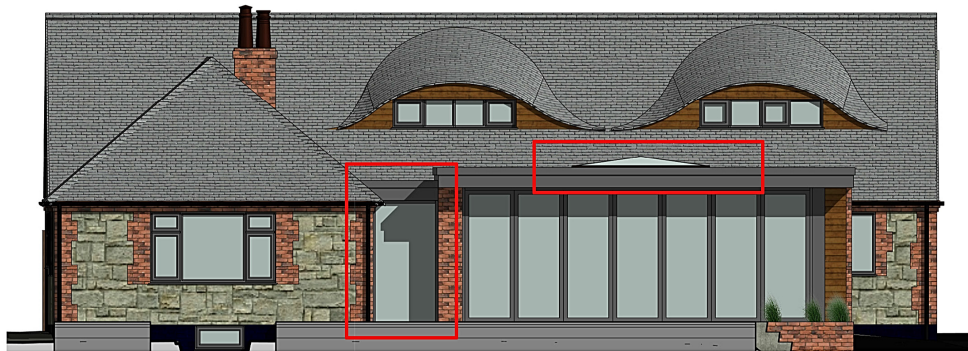
1 Proposed North Elevation - As Planning application ref: 9/2019/0264 1:50
