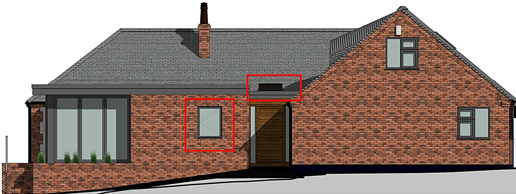
2 Proposed West Elevation - As Planning application ref: 9/2019/0264 1:50
