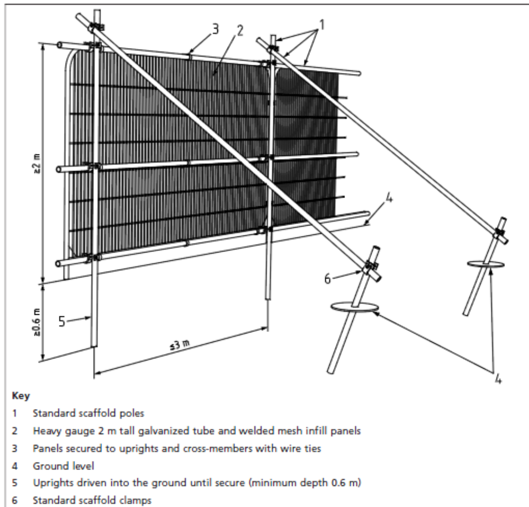
Figure 1 - Tree Protection Barrier
