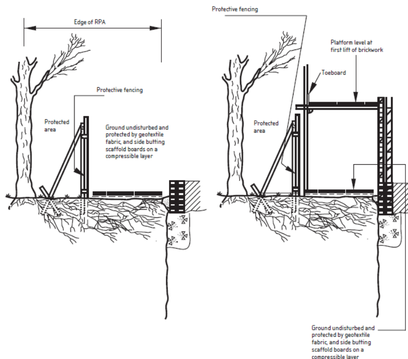
Figure 3 Adapted Barrier Incorporating Temporary Ground Protection
