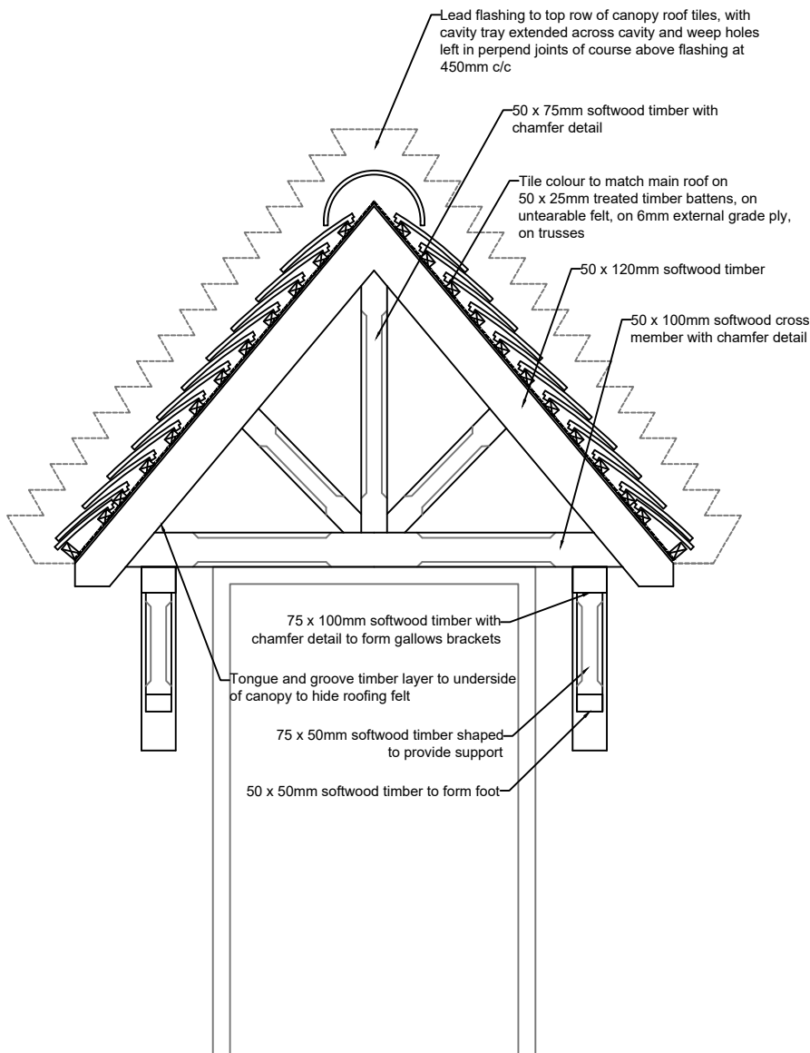
Detail Elevation
