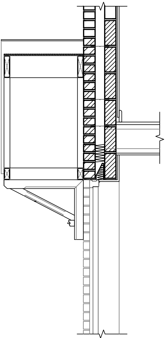
Detail Section
