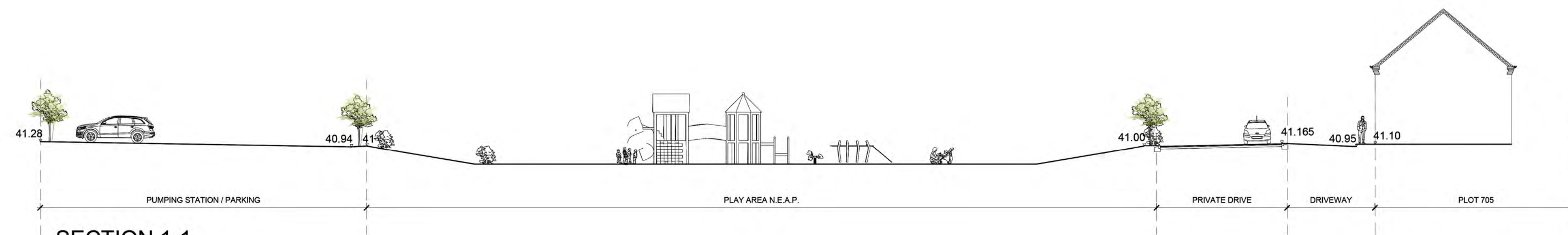
SECTION 1-1
