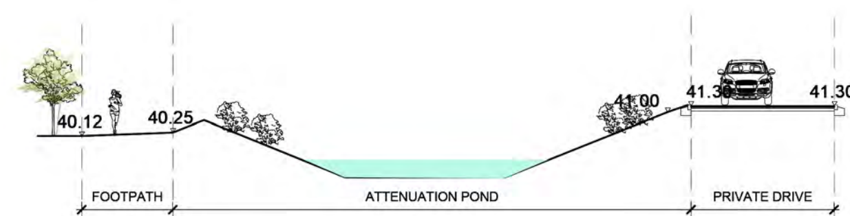
SECTION 5-5
