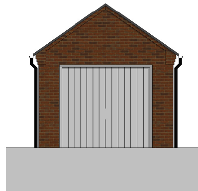
Front Elevation 1 : 100
