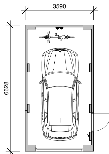
Single Floor Plan 1 : 100
