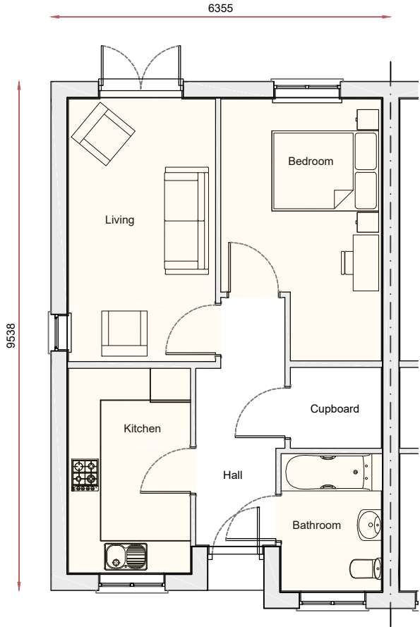
FLOOR PLAN
