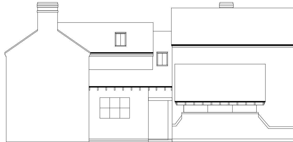
side (eastern) elevaion
