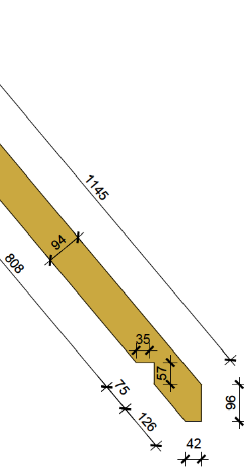
RAFTER [7] DETAIL SIZE: 94 X 70MM
