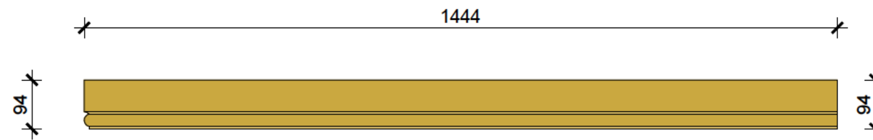
TORUS FASCIA [10] DETAIL SIZE: 94 X 19MM
