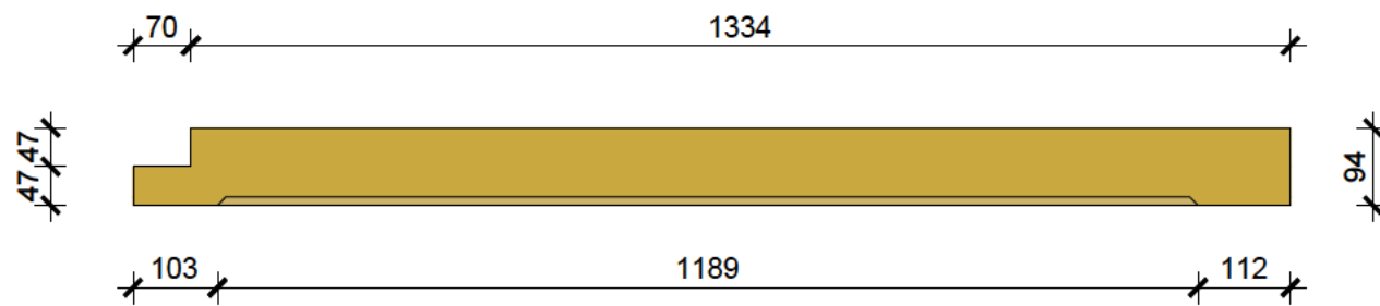
WALLPLATE [4] DETAIL SIZE: 94 X 70MM
