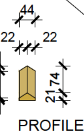
HIP RAFTER [8] DETAIL SIZE: 94 X 44MM
