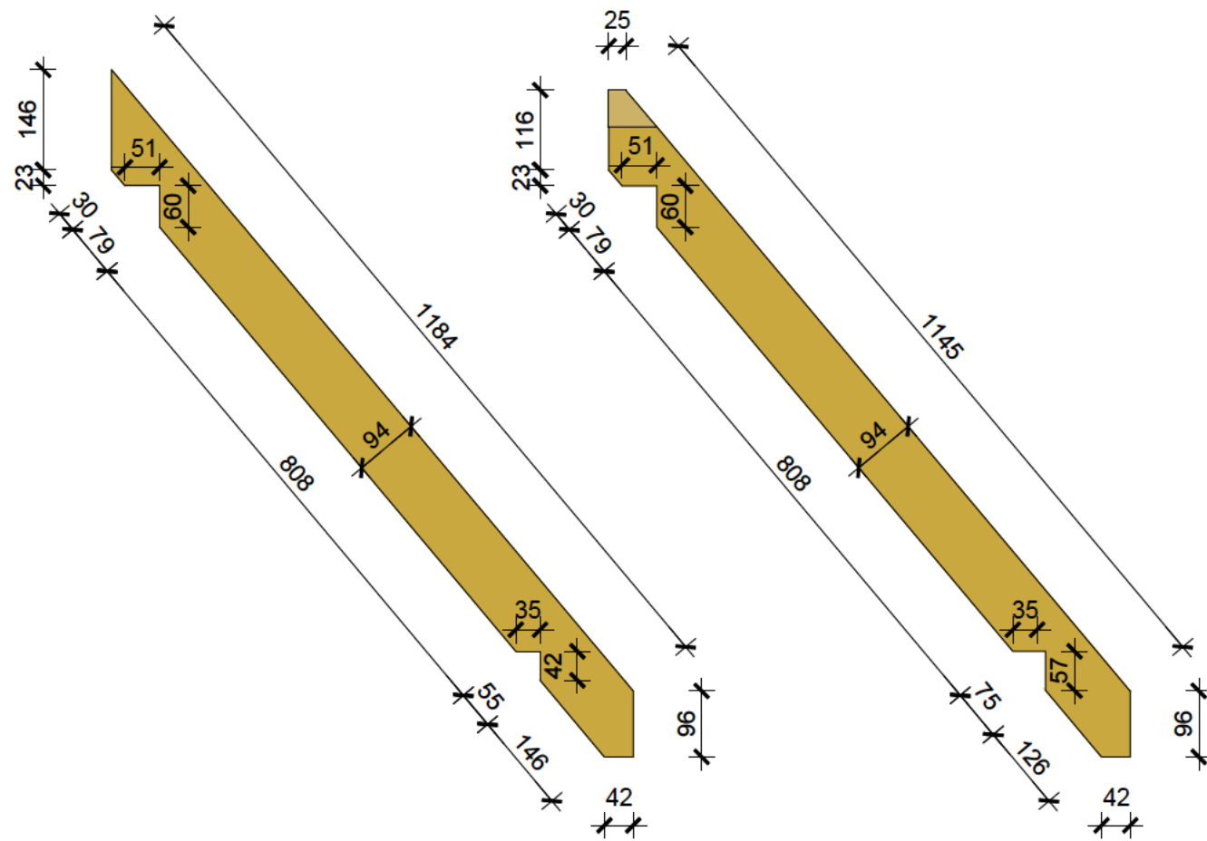
RAFTER [6] DETAIL SIZE: 94 X 70MM
