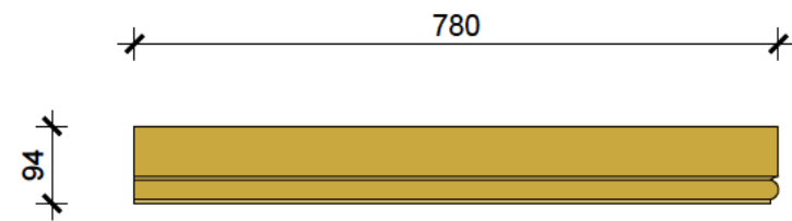
TORUS FASCIA [11] DETAIL SIZE: 94 X 19MM
