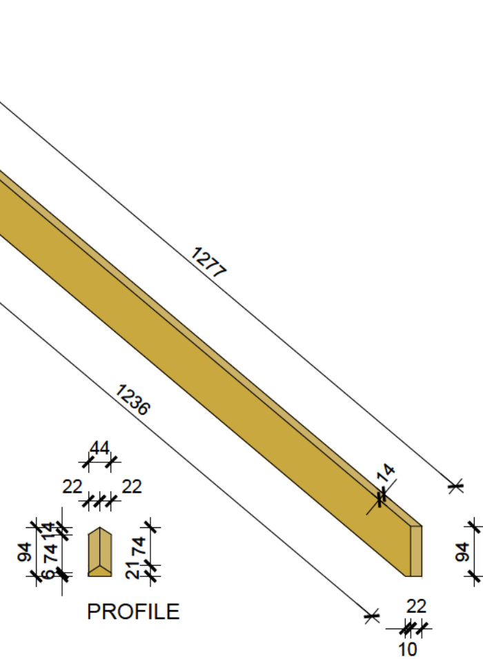
HIP RAFTER [8] DETAIL SIZE: 94 X 44MM
