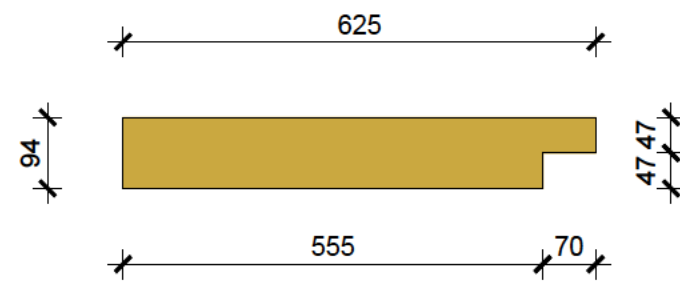
WALLPLATE [5] DETAIL SIZE: 94 X 70MM
