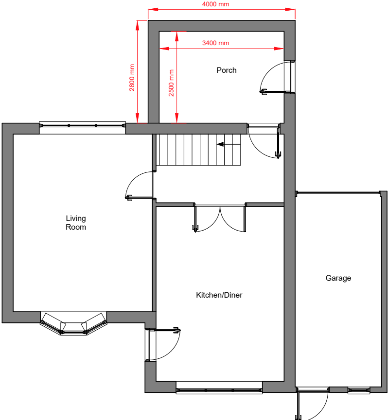
Proposed GF Plan
