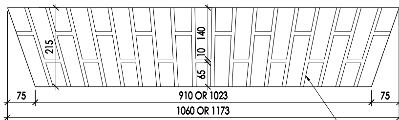
FRONT ELEVATIONS
