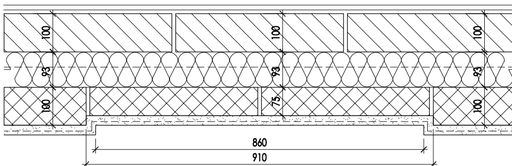
RENDER FALSE WINDOW RECESS PANEL
