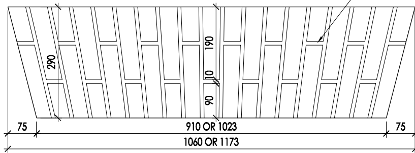
FRONT ELEVATIONS
