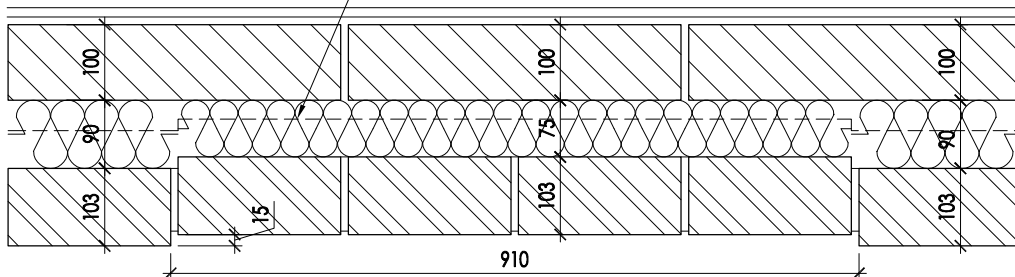
BRICK FALSE WINDOW RECESS PANEL
