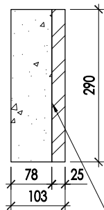
SECTIONS
