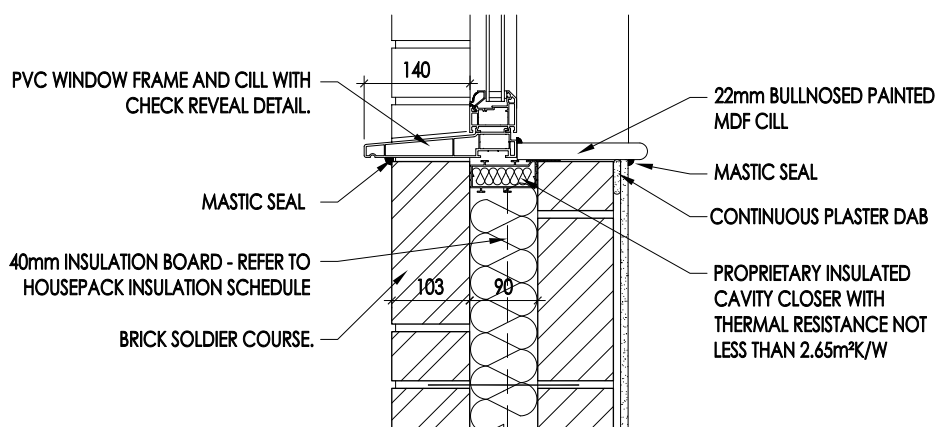
STANDARD HEADER DETAIL
