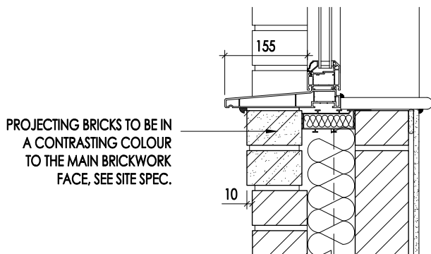
BRICK FEATURE BAND DETAIL
