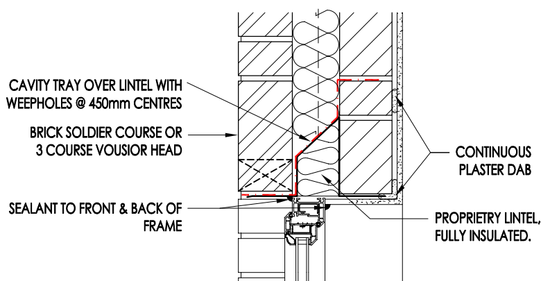
STANDARD BRICK SOLDIER OR 3 COURSE VOUSIOR DETAIL
