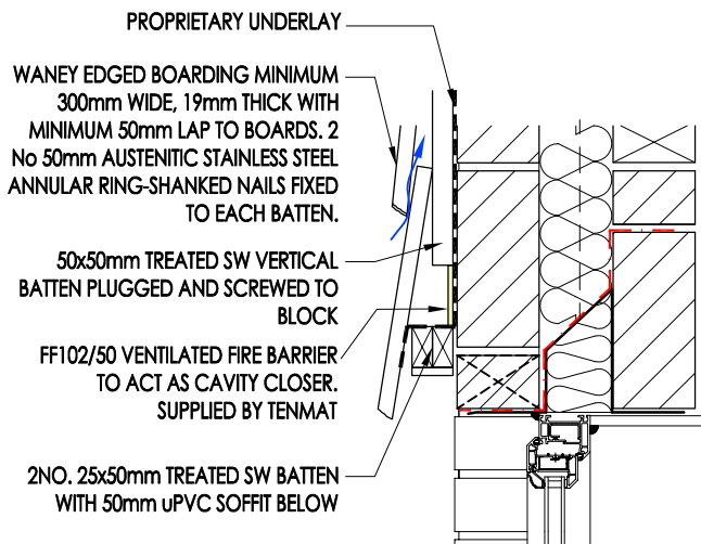
WANAY EDGE BOARD DETAIL
