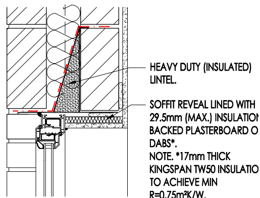
HEAVY DUTY LINTEL DETAIL - APPLIES TO ALL THE ABOVE DETAILS WHEN A LINTEL WITH CONTINUOUS BASE PLATE IS REQUIRED
