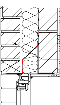
BRICK QUOIN DETAIL
