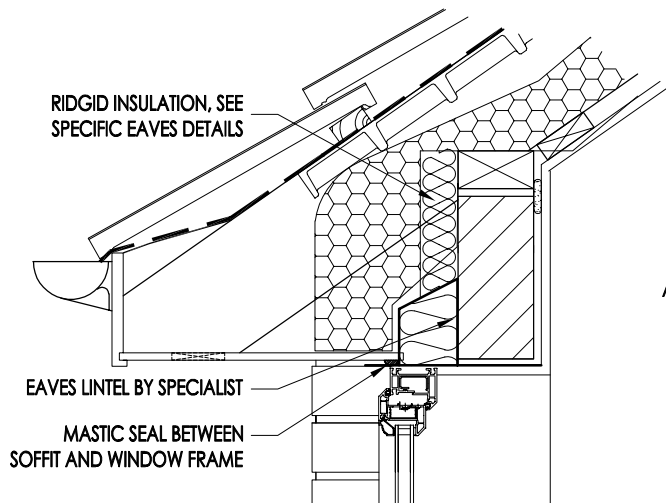
DROPPED EAVES SOFFIT DETAIL
