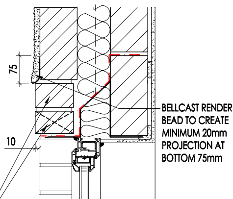
BRICK BANDING/RENDER DETAIL
