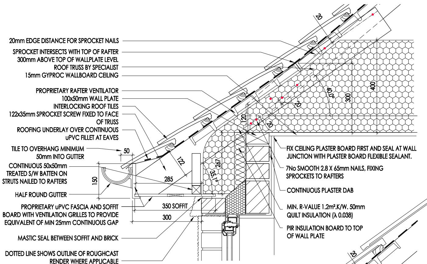
40°/35.1° SPROCKET EAVES DETAIL (DUO-PLAIN TYPE TILE)
