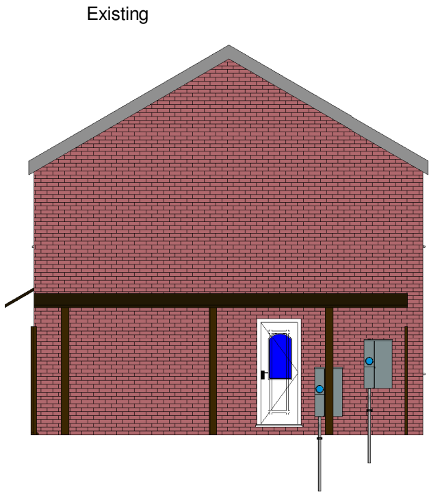
2 Side A Elevations 1 : 100
