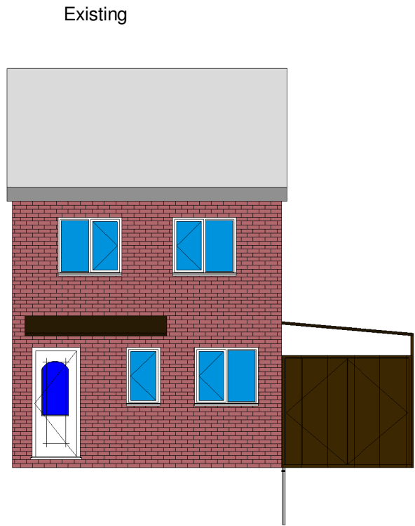
1 Front Elevations 1 : 100
