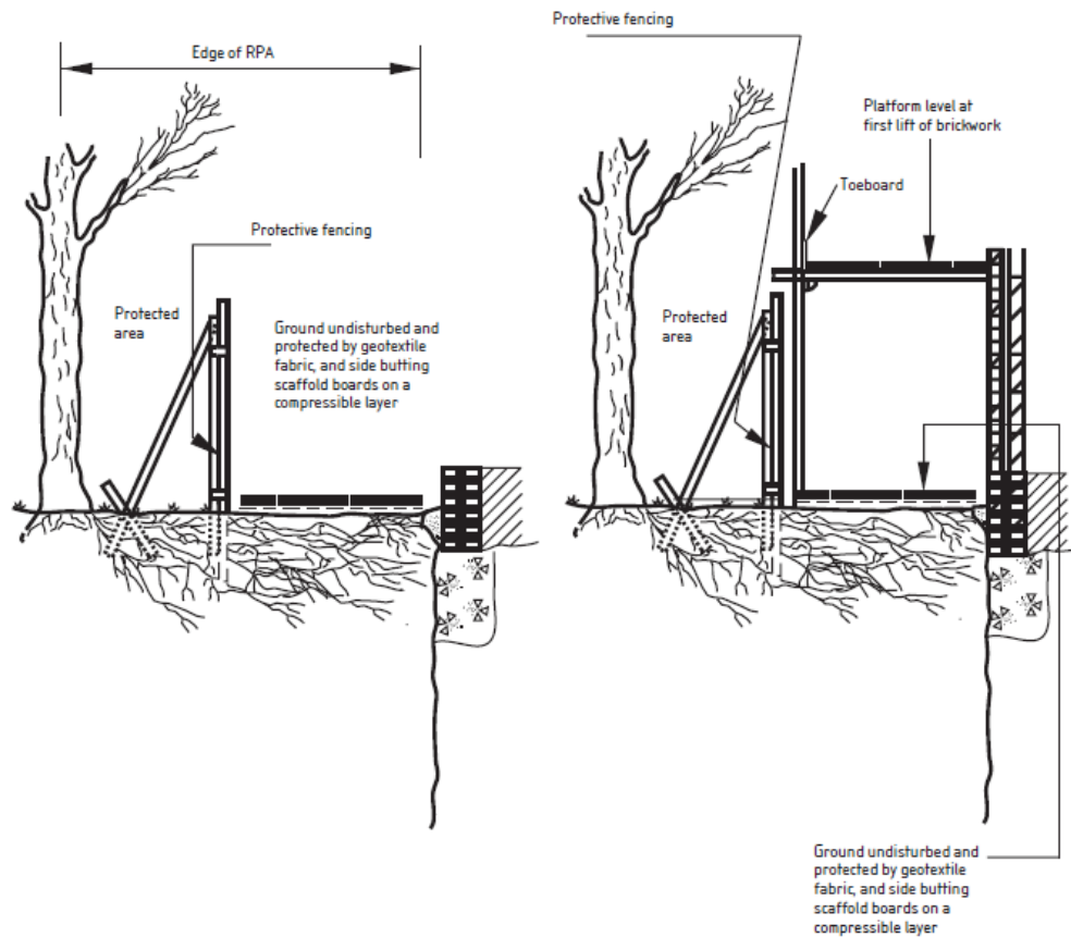
Figure 2 Adapted Barrier Incorporating Temporary Ground Protection
