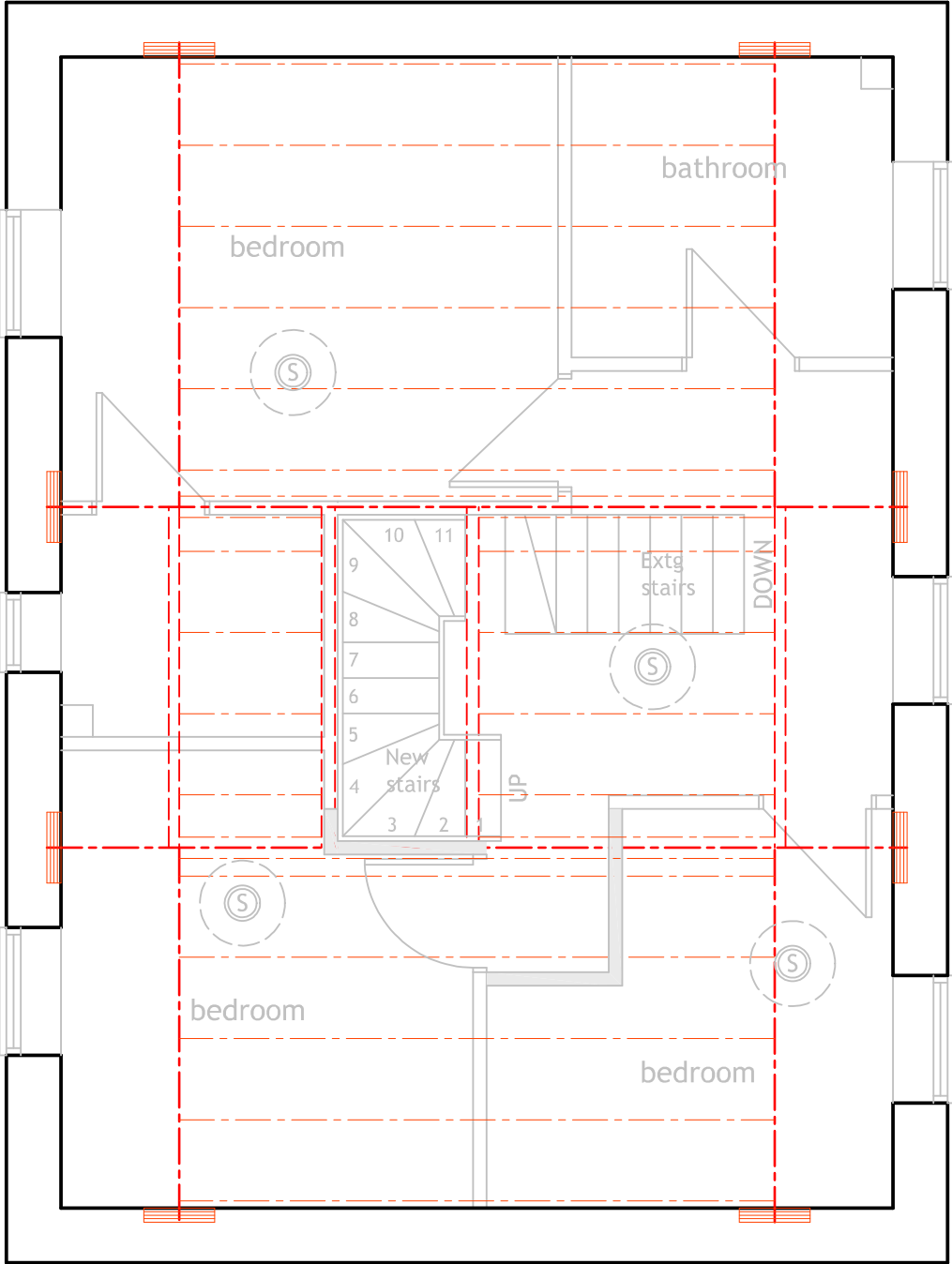
PROPOSED FIRST FLOOR PLAN - LOFT FLOOR CONSTRUCTION SUPERIMPOSED -
