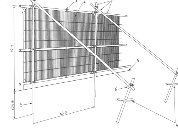
Figure 1: Detail Specification for Protective Barrier.
