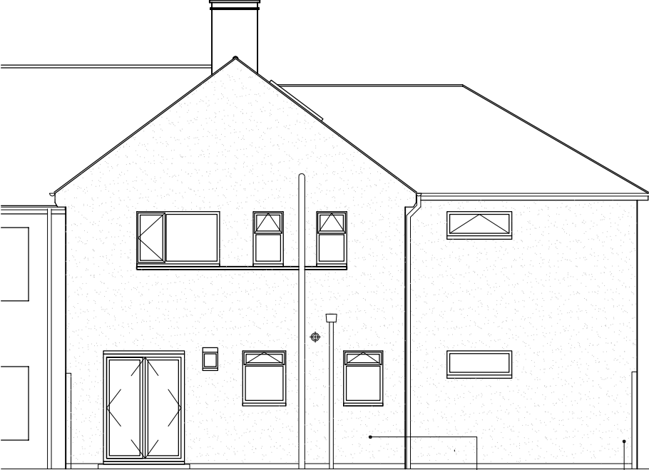
Proposed Reart Elevation
