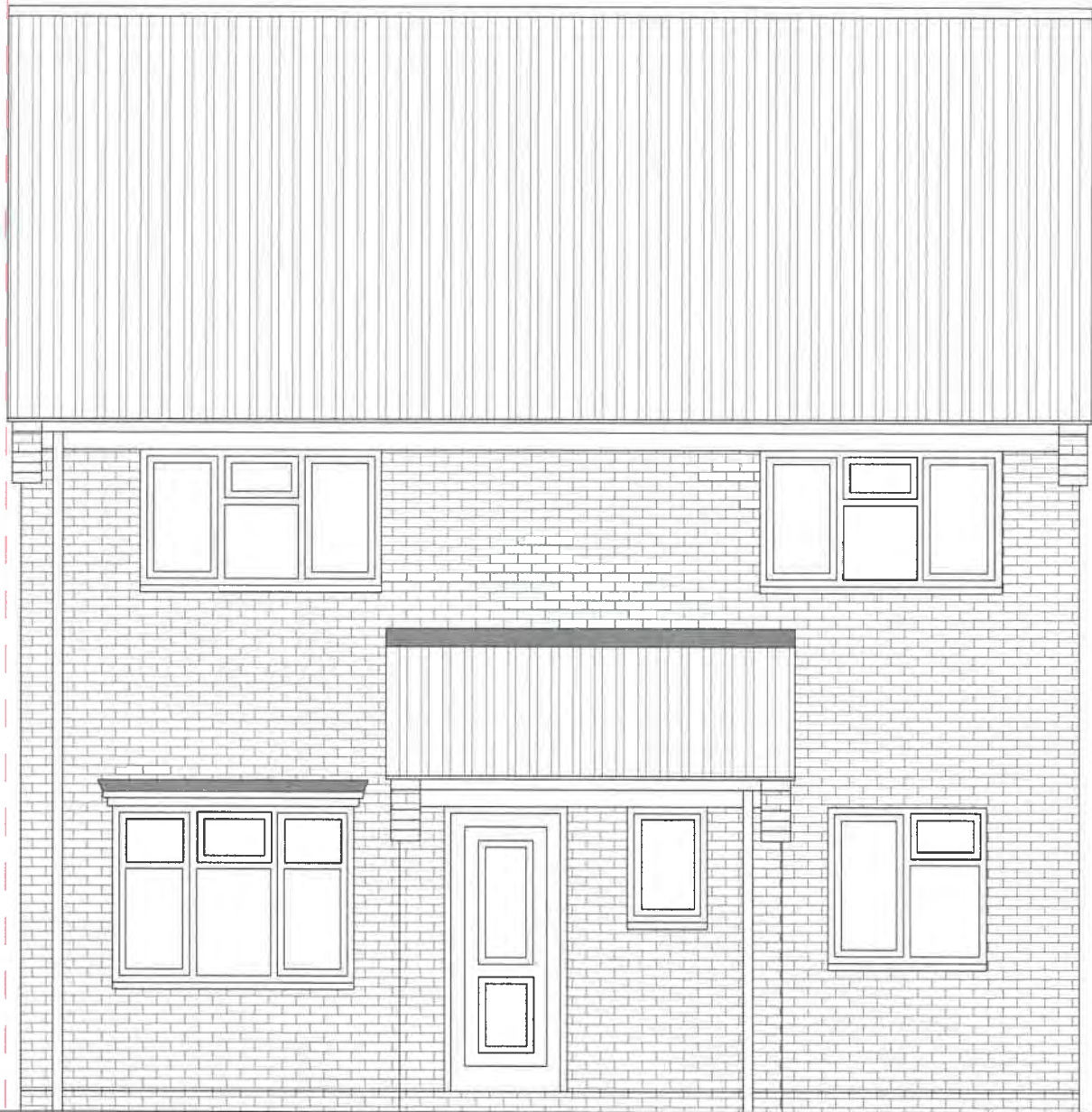
Existing Front Elevation. 1:50 at A3
