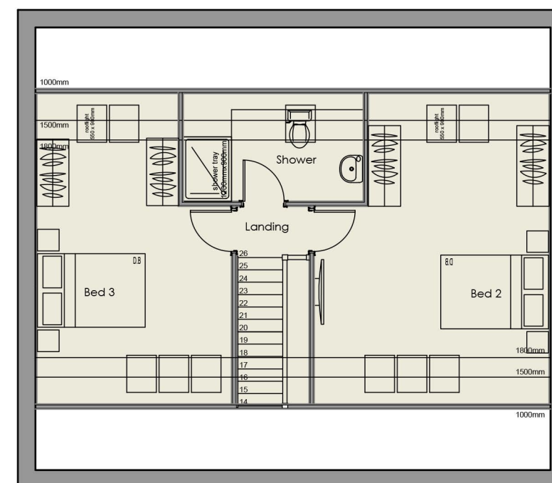
Second Floor Plan 45.4 sq.m (upto 1500mm high)
