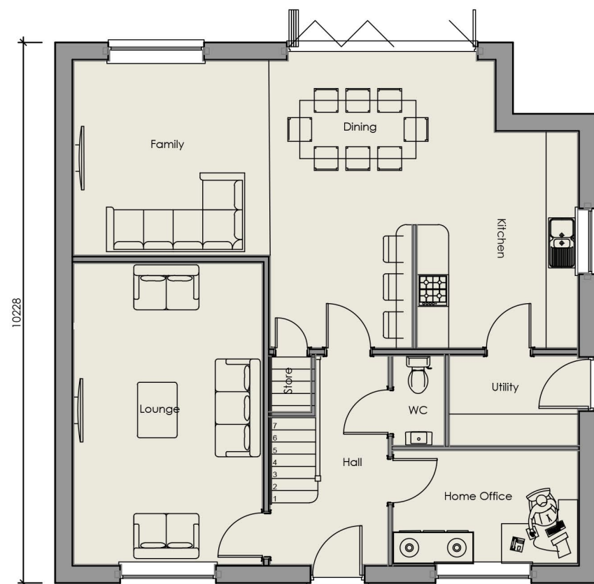
Ground Floor Plan 89.2 sq.m
