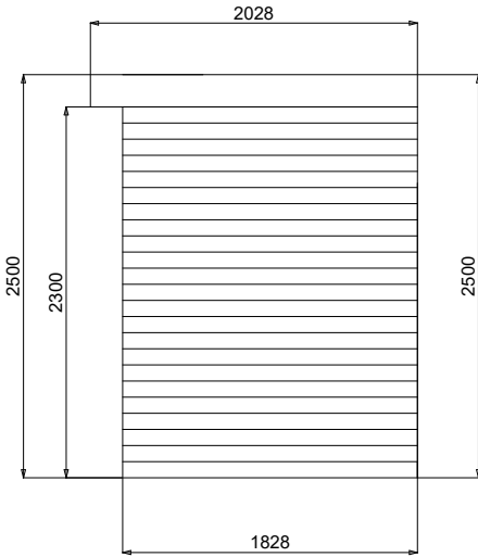
SIDE ELEVATIONS
