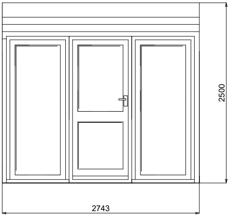
FRONT ELEVATION
