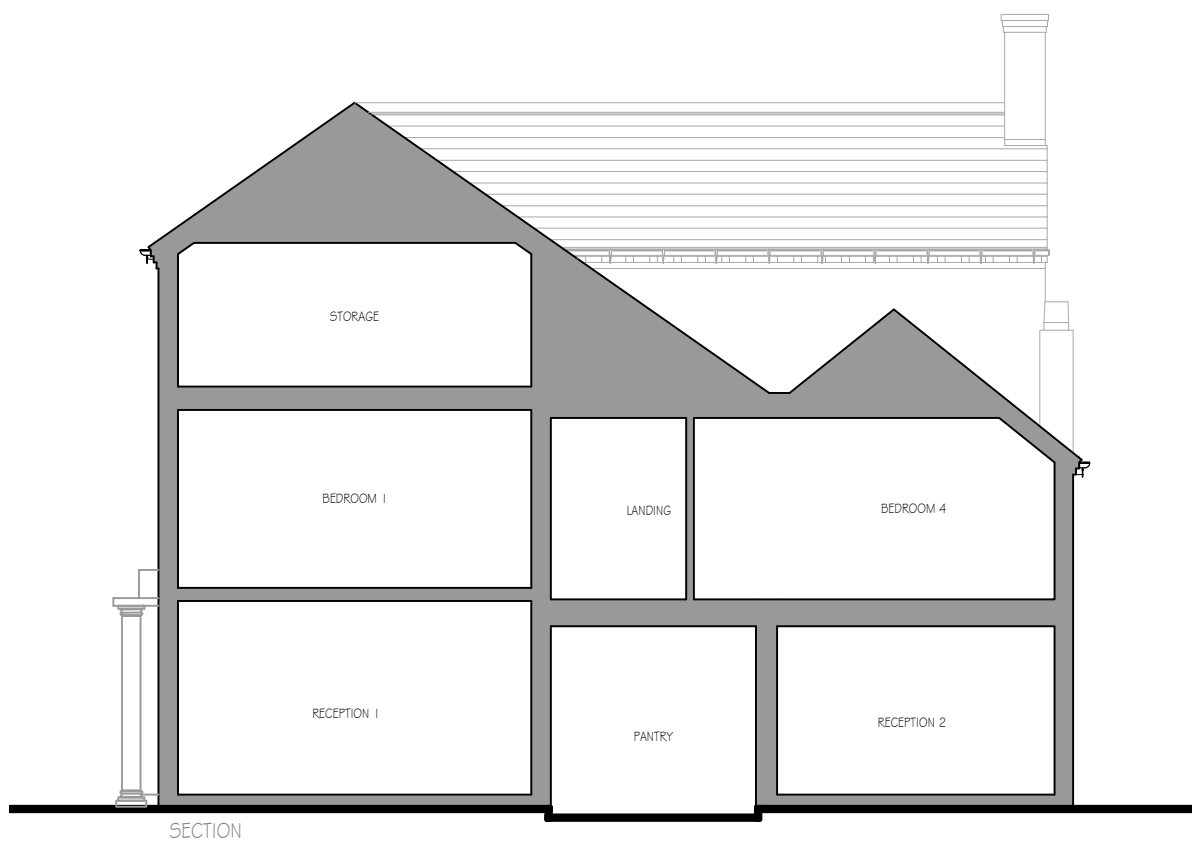
SECTION
