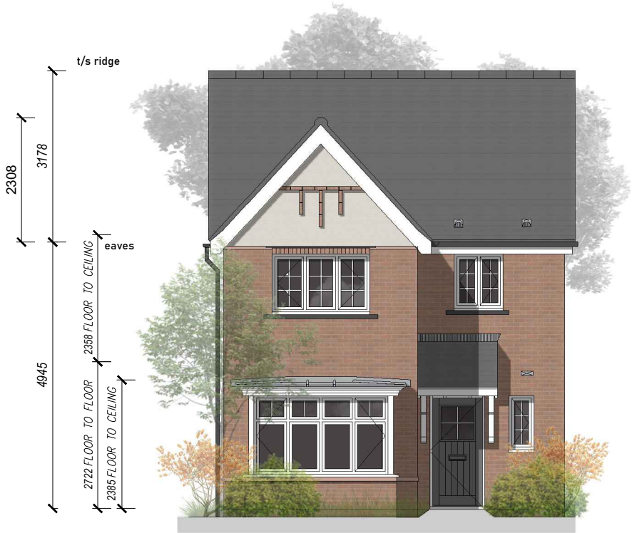
FRONT ELEVATION
