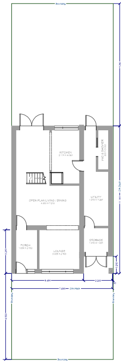
Proposed Ground Floor Plan
