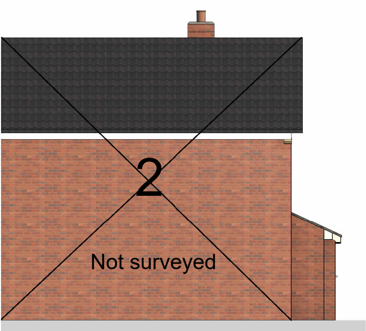
Proposed Side Elevation (No.2) 1 : 100
