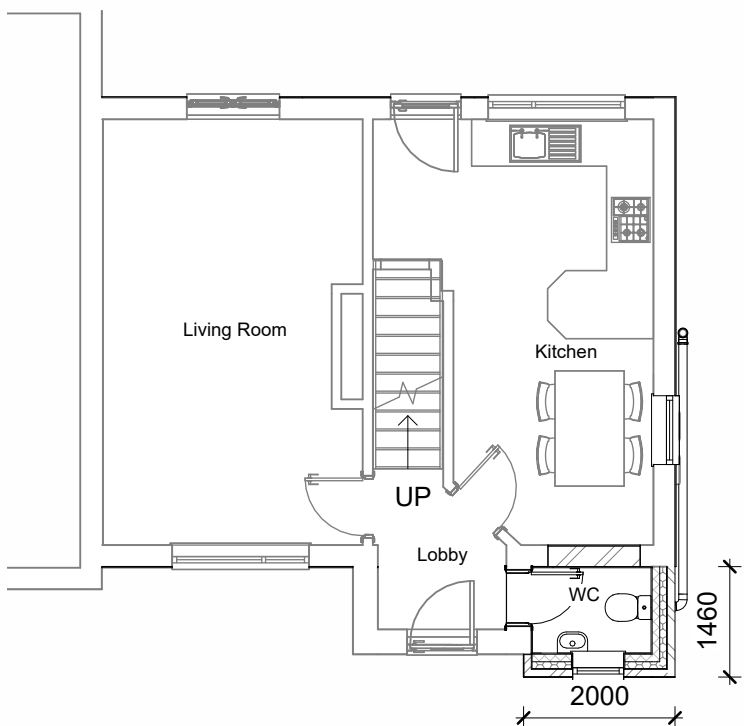
Proposed Ground Floor Plan 1 : 100
