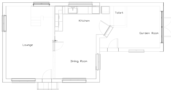
Ground Floor Plan as Existing
