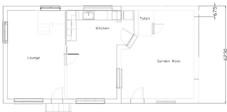
Ground Floor Plan Proposed
