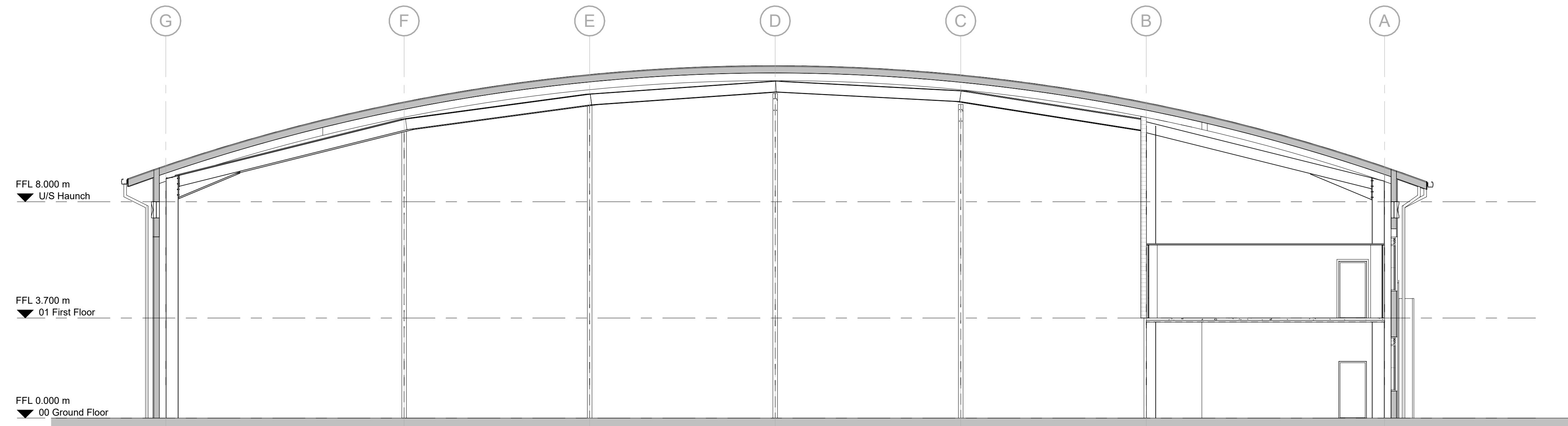
B Plot 3b Proposed Section B-B Scale @ 1 : 100
