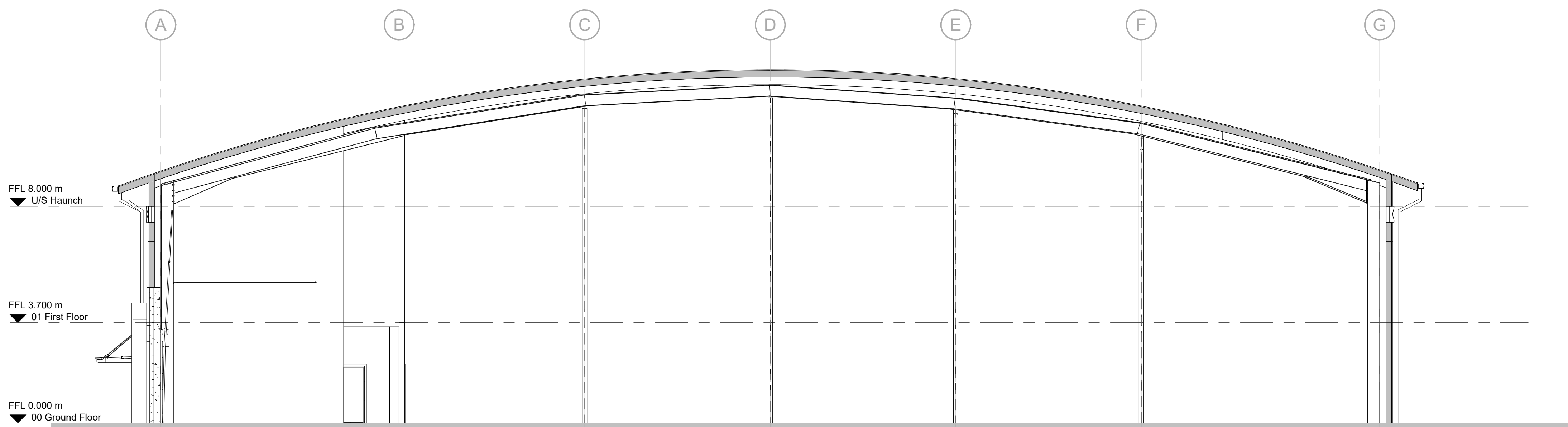
A Plot 3b Proposed Section A-A Scale @ 1 : 100
