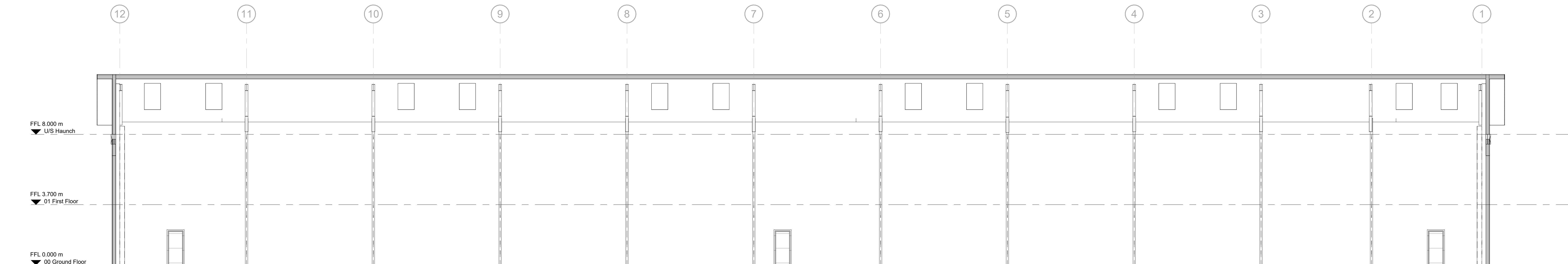
D Plot 3b Proposed Section D-D Scale @ 1 : 100
