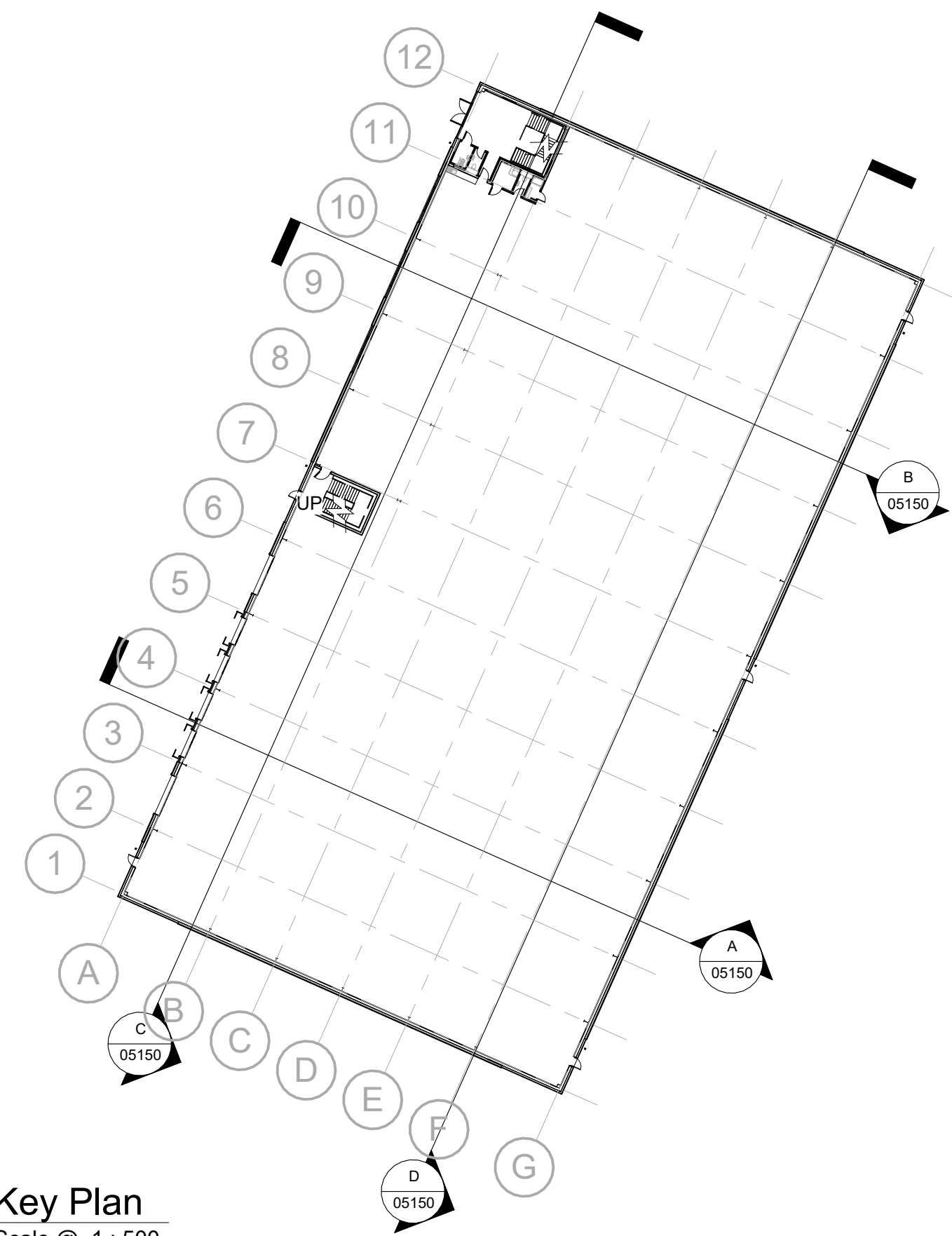
Key Plan Scale @ 1 : 500
