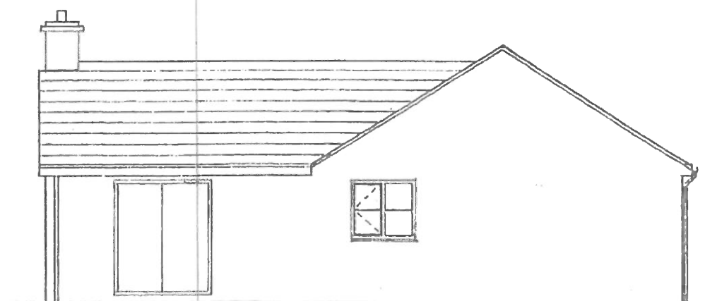
Proposed Rear Elevation C
