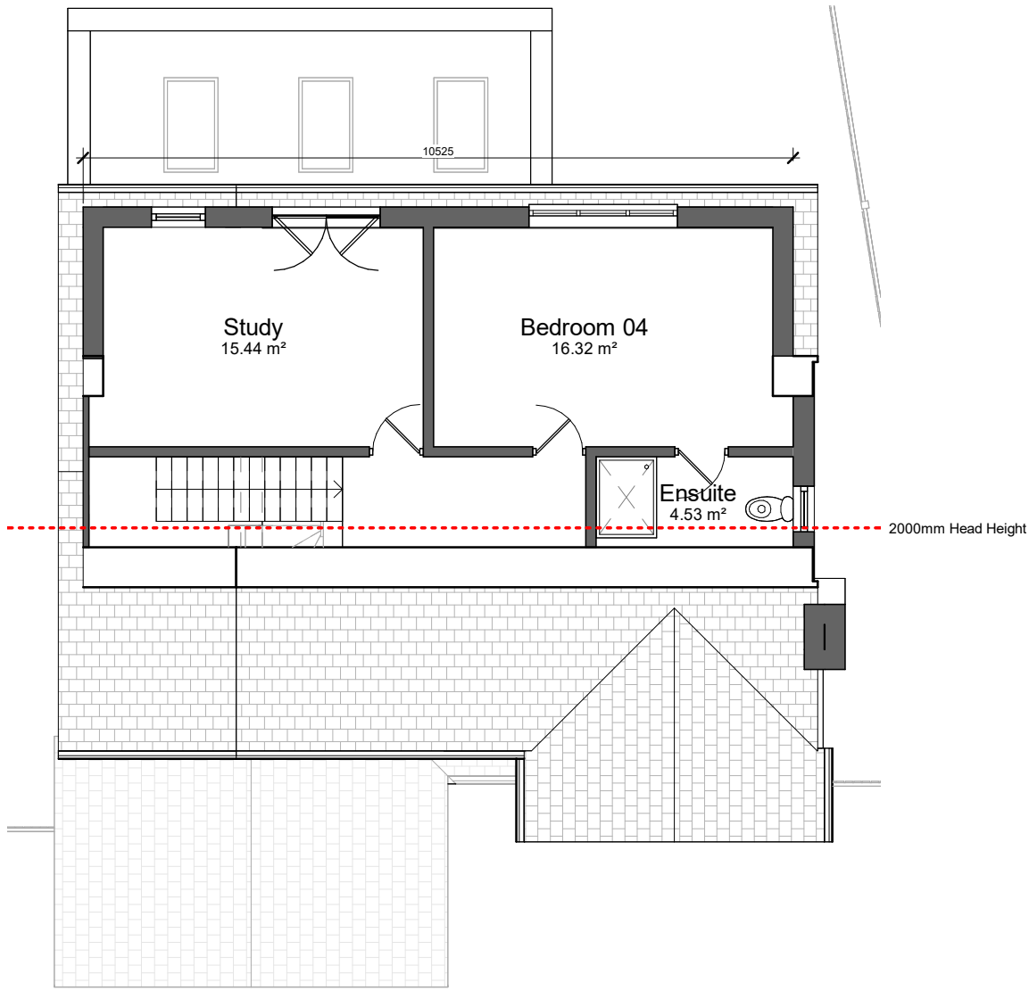
Proposed Loft Floor Plan Scale 1 : 100
