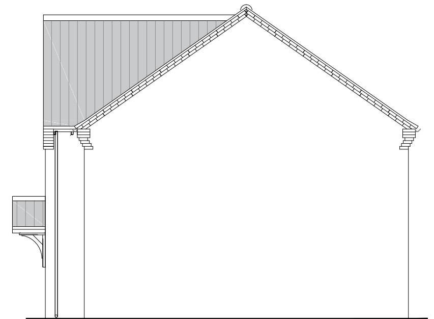
Side Elevation
