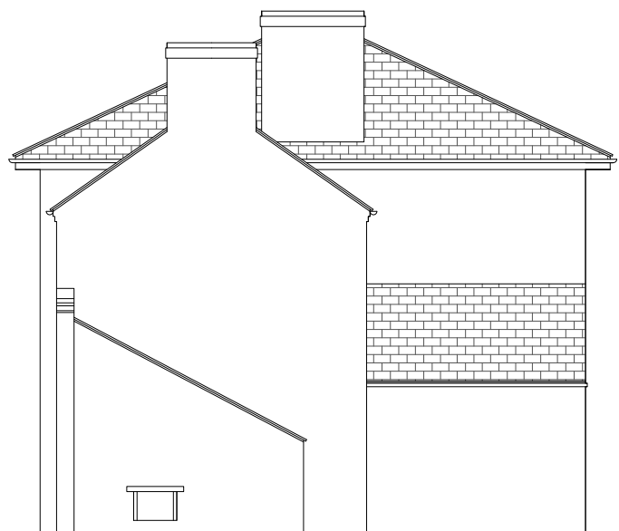
East Elevation
