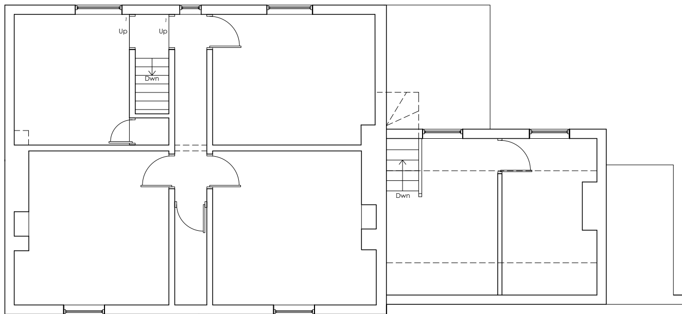
First Floor
