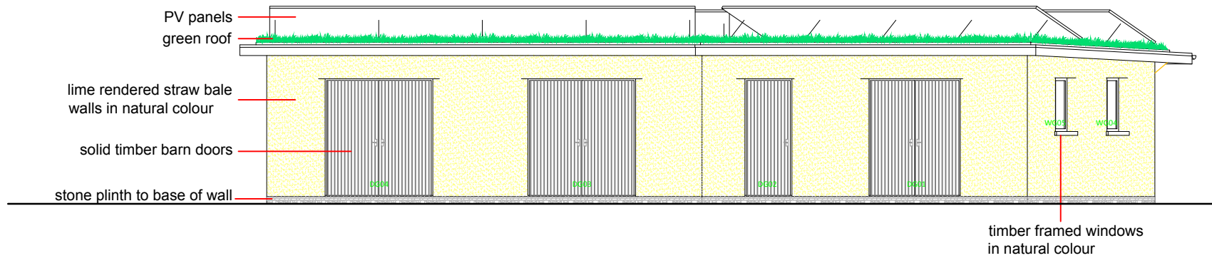
North Elevation
