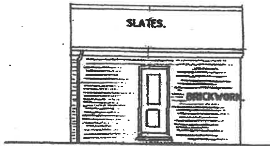
SHOWER BLOCK FRONT ELEVATION
