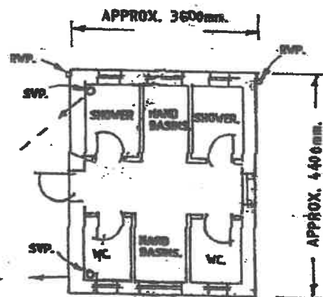
PROPOSED SHOWER BLOCK
