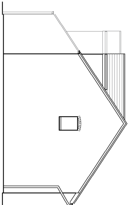
north elevation | as existing
