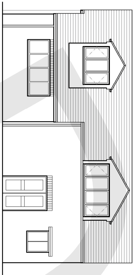
east elevation | as existing
