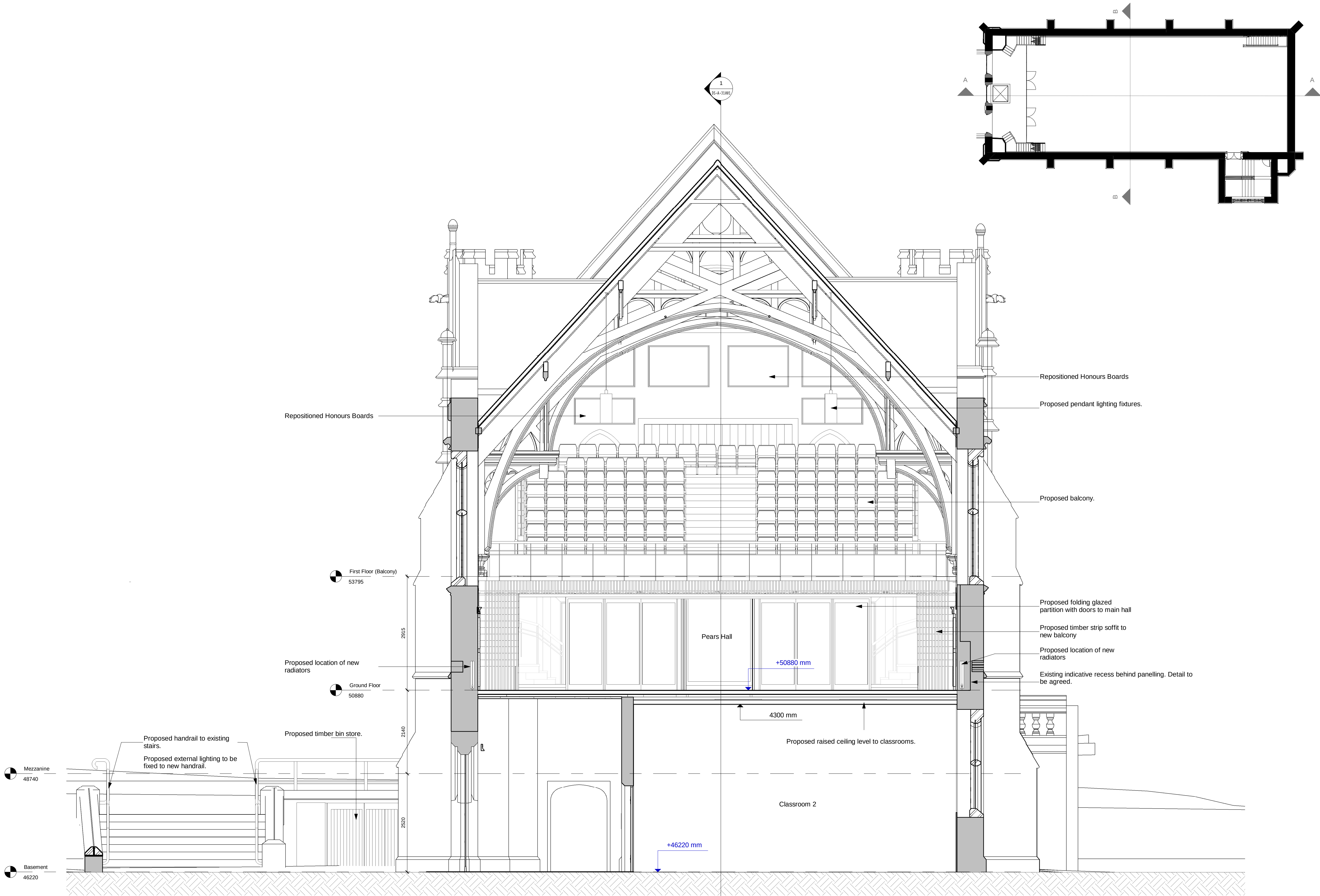
1 Proposed Section BB 1 : 50
